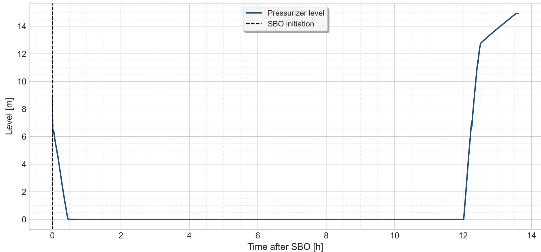
Base Case - Pressurizer Level
